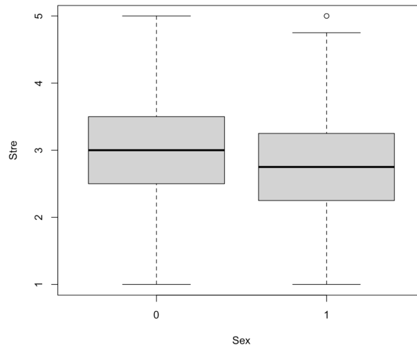
Figure 4.4: Boxplot
